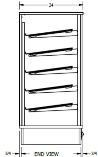
END VIEW
