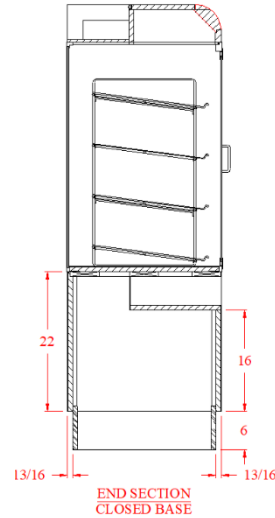
END SECTION CLOSED BASE
