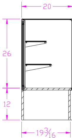
Side Elevation
