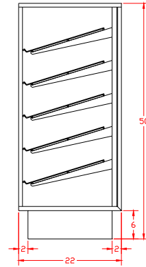
END VIEW
