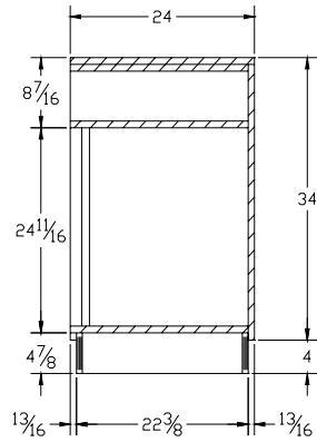
SIDE ELEVATION
